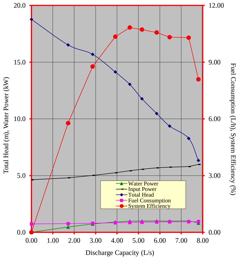
Figure 3. Performance characteristic curves of the KATO KDP50 self-priming centrifugal pumpset
